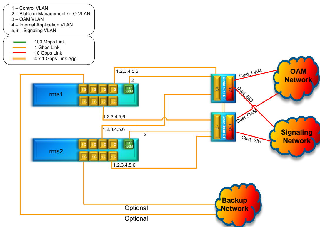
Figure 1: Logical Diagram of HP DL380 GEN 8 / GEN 9 RMS deployment using aggregation switches(L2/L3 Demarcation)
